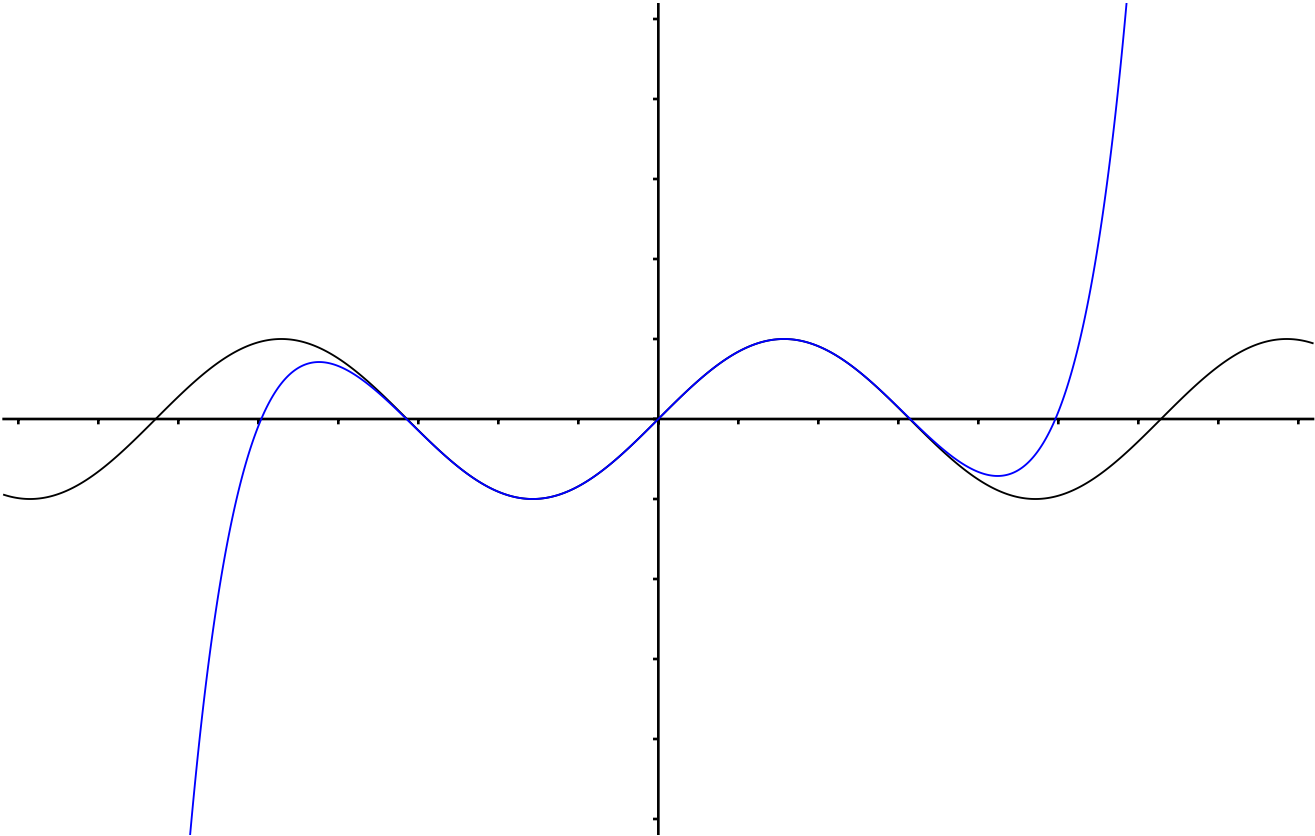
Taylor Polynomial for \sin(x) with degree 9
