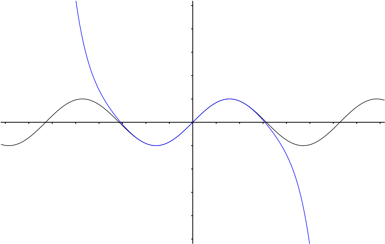
Taylor Polynomial for \sin(x) with degree 7
