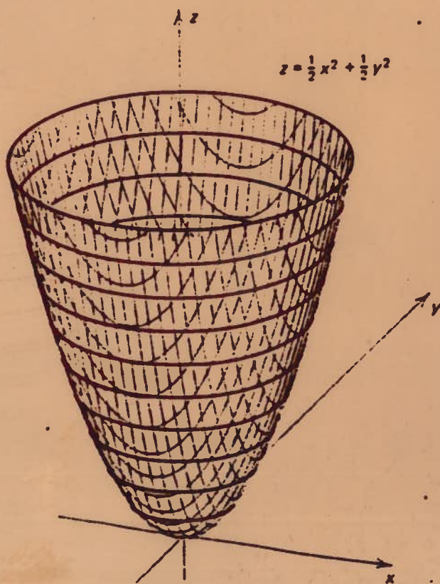
FIGURE 13.12 Horizontal cross sections of z = \frac{1}{2}x^2 + \frac{1}{2}y^2
