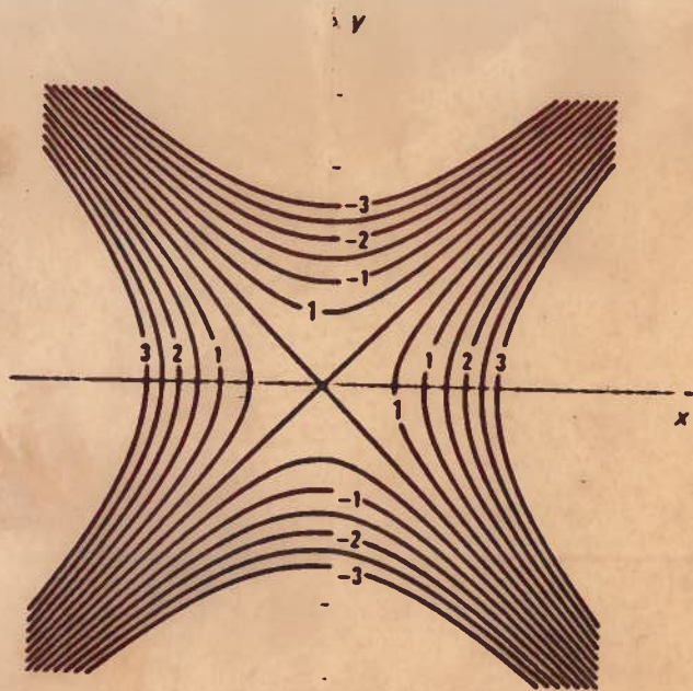
FIGURE 13.13 Level curves of \frac{1}{2}x^2 - \frac{1}{2}y^2
