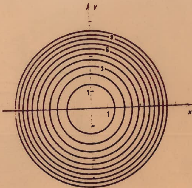
FIGURE 13.11 Level curves of \frac{1}{2}x^2 + \frac{1}{2}y^2
